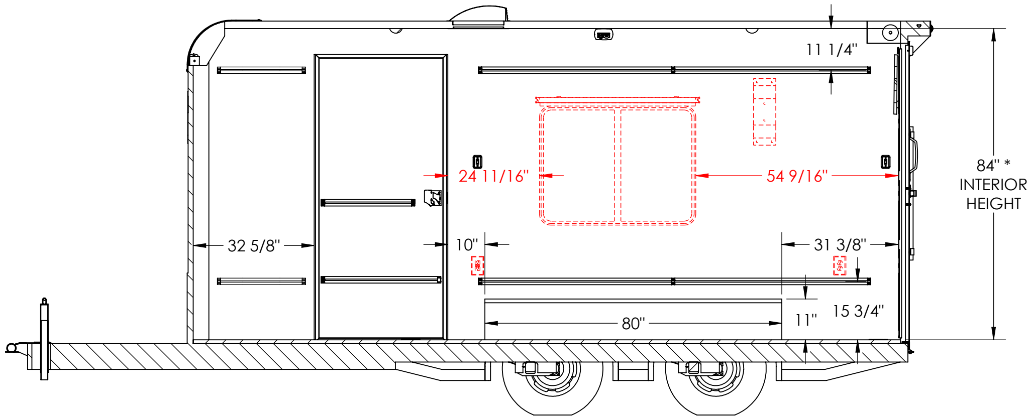
INTERIOR CURB SIDE SECTION B-B
