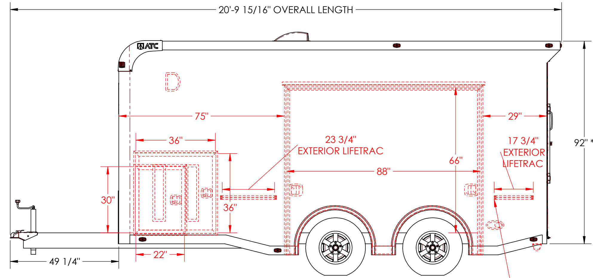
EXTERIOR CURB SIDE
