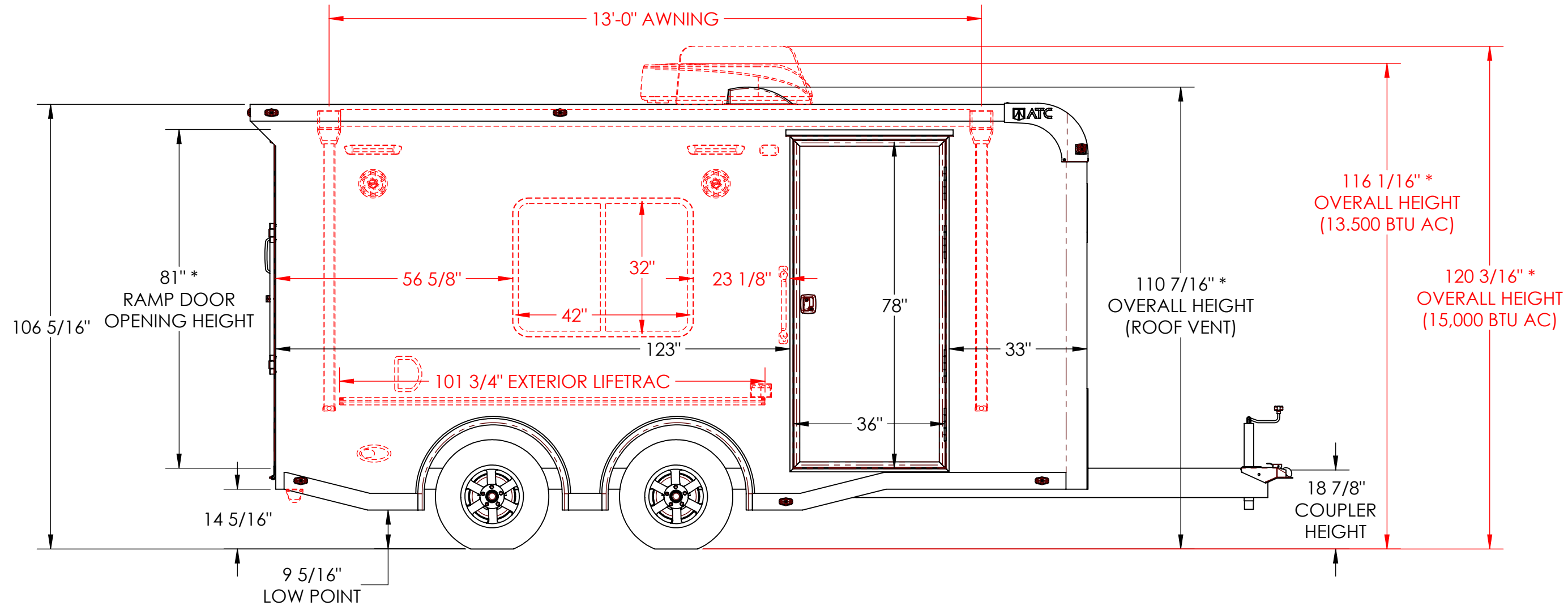
EXTERIOR ROAD SIDE
